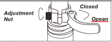
Fig.8 Opening and adjusting a quick release
